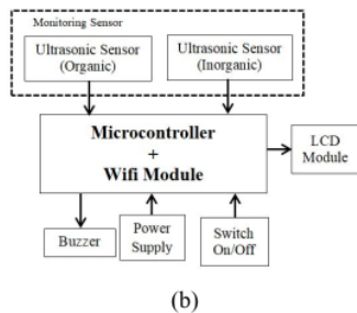
Fig. 1. Block Diagram of G-Bot One
