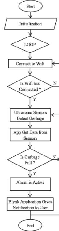
Fig. 5. Flowchart of the G-Bot
