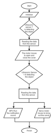
Figure 3. Flowchart of G-Box System
