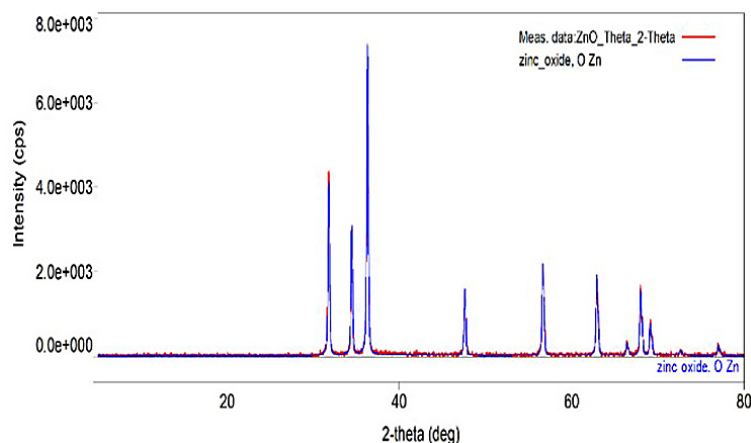
Figure 2. XRD sample result
