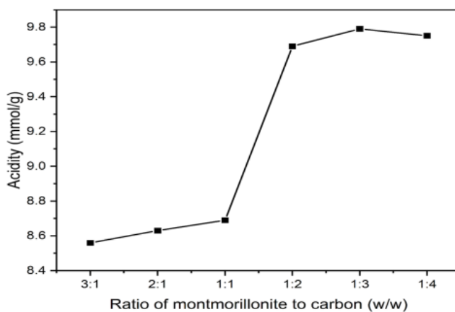
78 Figure 2. Effect of ratio of montmorillonite to carbon (% w/w) on catalyst acidity
