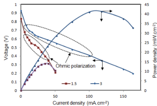
Figure 1. The comparison of the performance of MEA with different carbon powder content in MPL ( \text{mg cm}^{-2} ).
