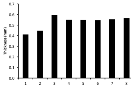
Figure 6. The thickness of the various MEA (1) Casting Method; (2) Commercial; (3) The method of spraying single layer; (4) 0.1 \text{ mg cm}^{-2} ; (5) 0.3 \text{ mg cm}^{-2} ; (6) 0.5 \text{ mg cm}^{-2} ; (7) 0.7 \text{ mg cm}^{-2} ; (8) 0.9 \text{ mg cm}^{-2} (numbers 4-8 were spraying method with three layers with different catalyst content)
