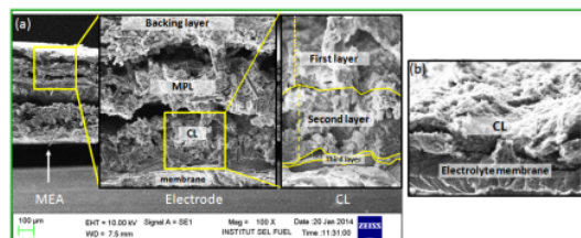
Figure 5. SEM image of a cross section of MEA, the electrode and the CL and CL cross-sectional comparison between the spray method (a) three-layer and (b) single layer
