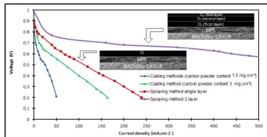
Figure 3. Comparison of the performance of the MEA between casting methods (containing carbon powder 1.5 \text{ mg cm}^{-2} and 3 \text{ mg cm}^{-2} ), method of spraying with single layer and three layers of catalyst content 0.3 \text{ mg cm}^{-2}
