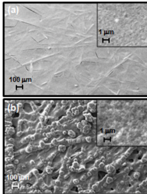
Figure 4. The comparison surface structure of MPL between casting method (a) and spraying method (b) with 100 x magnification (inset, 10,000x magnification).
