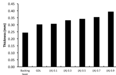
Figure 2. The thickness of BL, GDL and anode (A) at various catalyst content ( 0.1, 0.3, 0.5, 0.7 dan 0.9 \text{ mg cm}^{-2} )
