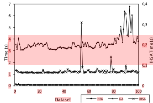
Fig. 8. Speed Comparison between IHSA, HSA and GA.
