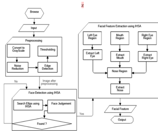
Fig. 5. Overall face detection and facial-feature extraction process.
