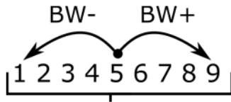
Fig. 12. Visualization of PAR and BW processes on harmony memory
