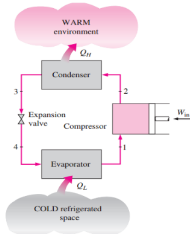
Figure 1. Refrigeration cycle
