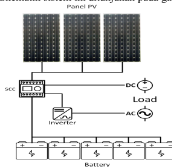
Gambar 5. Skema PLTS Off-Grid
