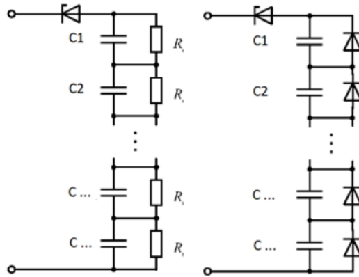
Figure 1 Circuitry scheme of EC module
