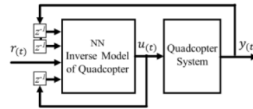
Fig. 4. Direct Inverse Control
