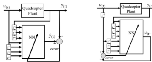
(a) Identification system (b) Inverse model
