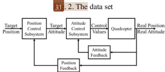
Fig. 3. Full control of quadcopter
