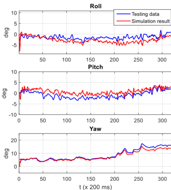
Fig. 7 Response result of attitude
