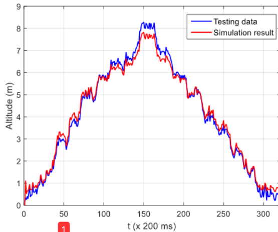
Fig. 6. Response result of altitude
