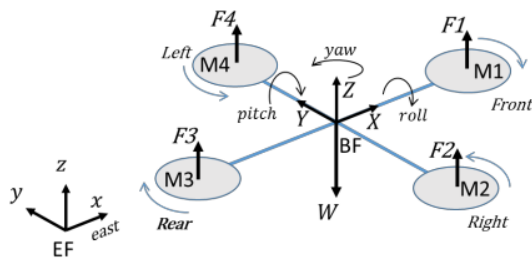
Fig. 1. Quadcopter basic movement
