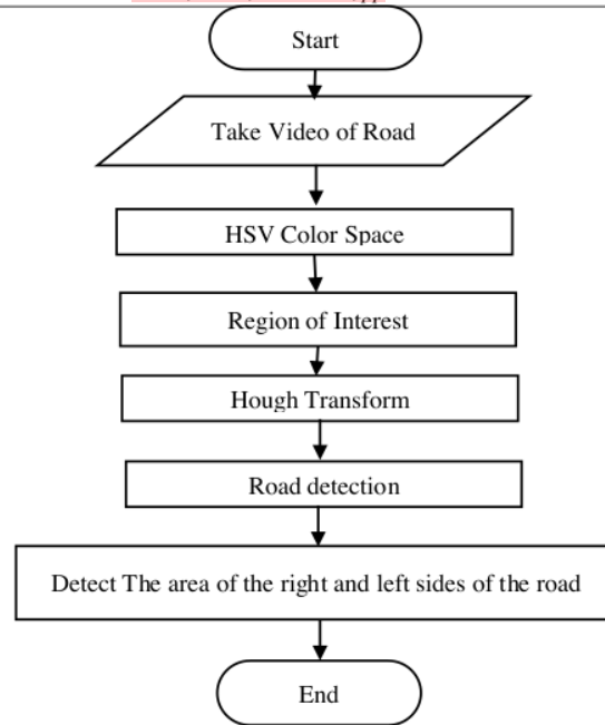
Fig. 2. Road detection flowchart
