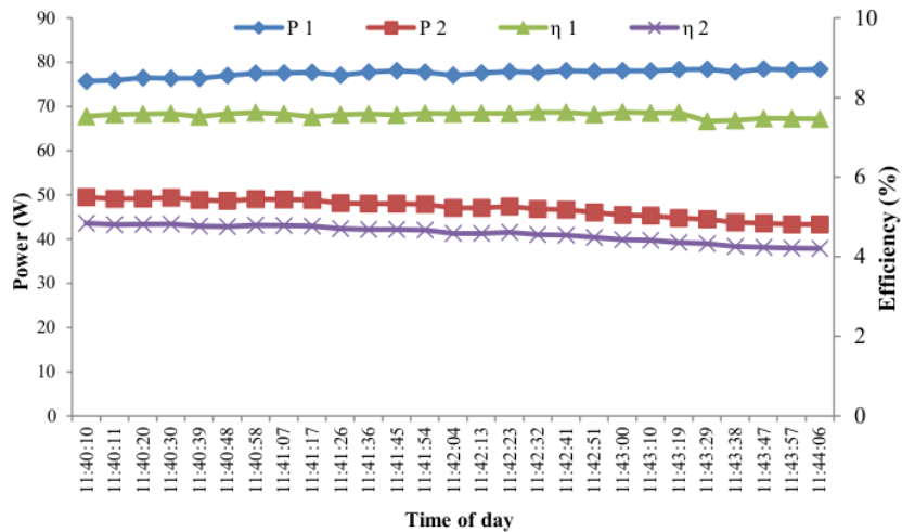
Figure 4. Comparison between power of PV panel using perforated plate (P 1) PV panel without perforated plate (P 2) and efficiency of PV panel using perforated plate ( \eta 1) PV panel without perforated plate ( \eta 2).
