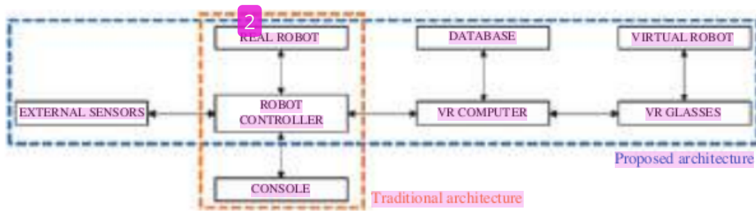
Figure 4.8 System architecture [41]
