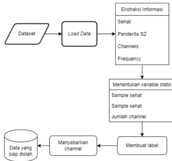
Diagram 2. Diagram tahapan preprocessing data.
