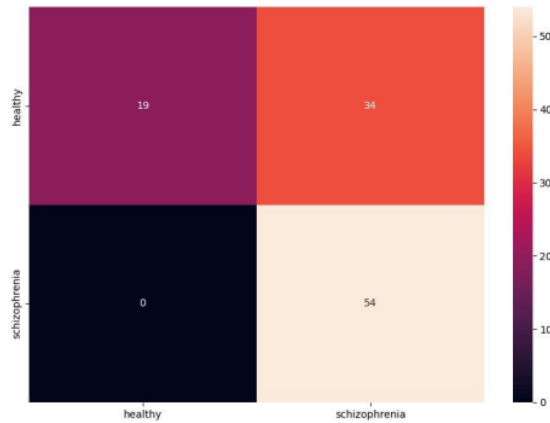
Gambar 3. Confusion Matrix Model CNN-LSTM Pertama
