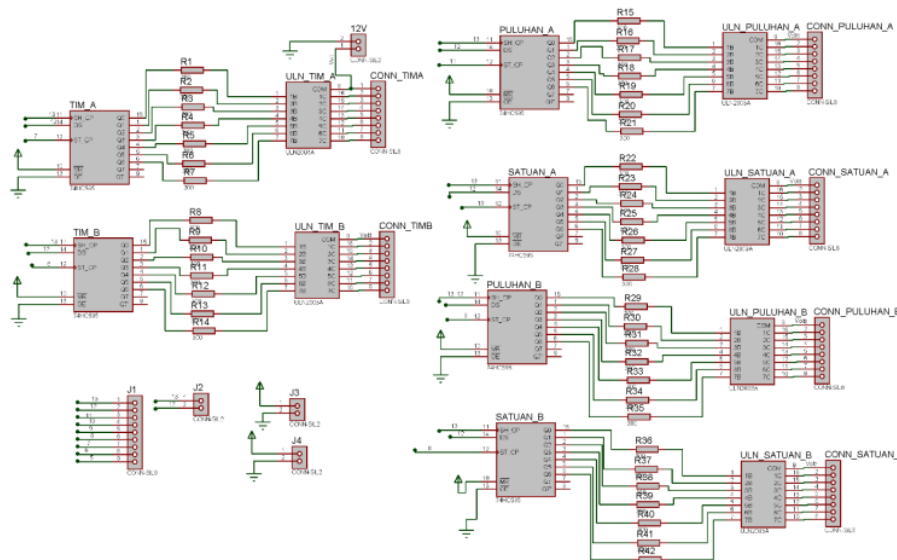
Gambar 1. Rangkaian scoreboard digital.
