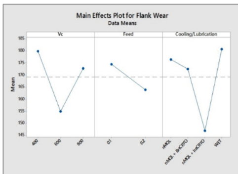
c) Average flank wear
