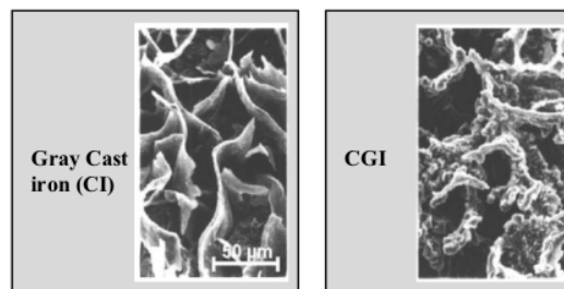
Fig. 1. Graphite particle shape of gray iron and compacted graphite iron [5]
