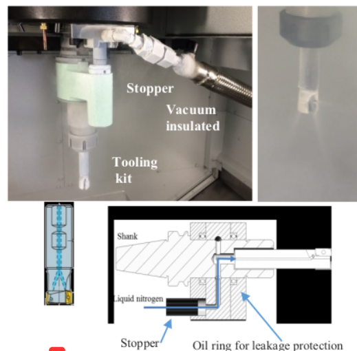
Fig. 3. Custom designed of internal cryogenic cooling tooling kit.
