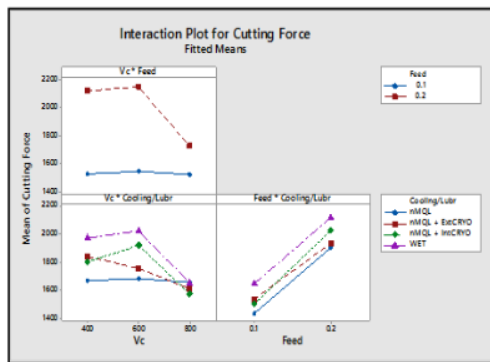
a) Cutting force
