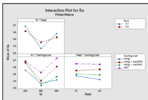
b) Surface roughness
