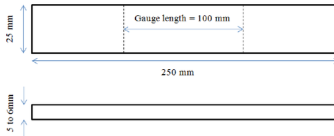
Figure 1. Specimen dimension
