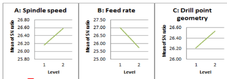
1 Figure 2. Taguchi response graph for residual tensile strength of BFRP composites
