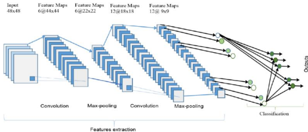
FIGURE 2. CNN Process
