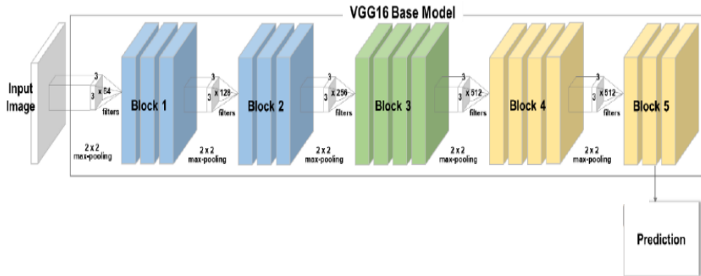
FIGURE 3. VGG-16 Architecture [27]
