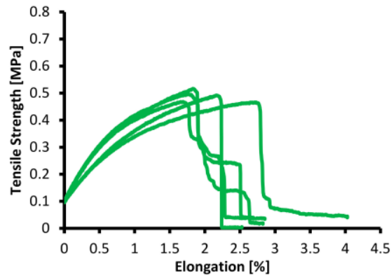
Figure 7. Tensile strength–elongation graph for 15 wt% PVDF with 1% tin dioxide.
