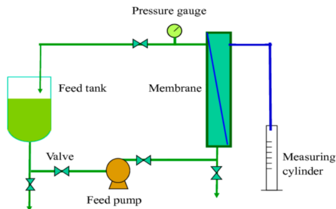
Figure 3. Schematic process of normalized water permeability.
