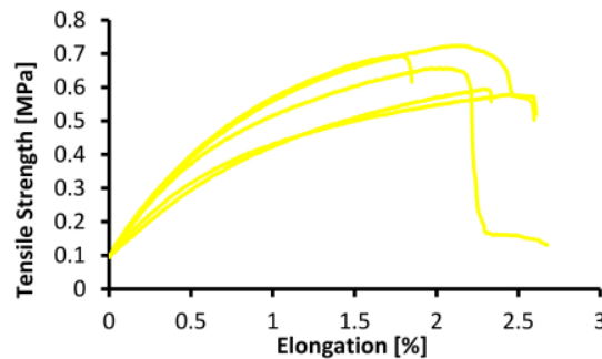
Figure 8. Tensile strength–elongation graph for 17.5 wt% PVDF with 1% tin dioxide.
