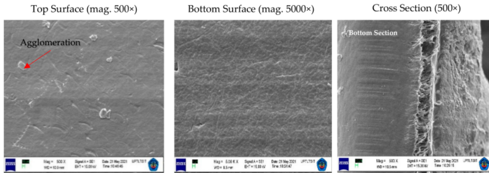
Figure 5. Structure of PVDF and tin dioxide membrane for 17.5 wt% PVDF with 1% tin dioxide. Top Section with Magnitude = 500×, WD = 10.0 mm, EHT = 15.00 kV, Signal A = SE1. Bottom Section with Magnitude = 5.00 K ×, Working Distance (WD) = 9.5 mm, EHT = 15.00 kV, Signal A = SE1. Cross Section with Magnitude = 500×, WD = 10.5 mm, EHT = 15.00 kV, Signal = SE1.
