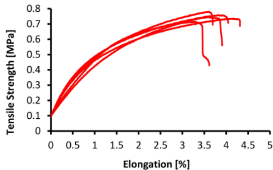
Figure 9. Tensile strength–elongation graph for 20 wt% PVDF with 1% tin dioxide.
