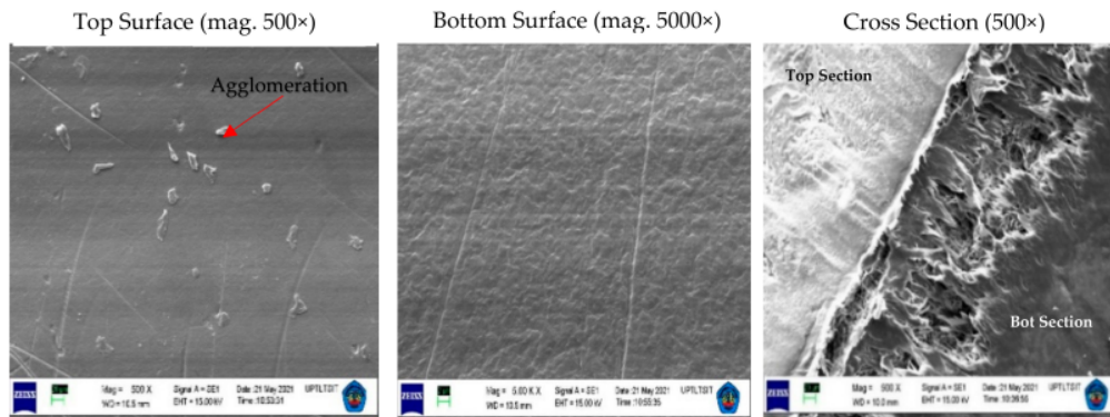
Figure 4. Structure of the PVDF and tin dioxide membrane for 15 wt% PVDF with 1% tin dioxide. Top Section with Magnitude = 500×, WD = 10.5 mm, EHT = 15.00 kV, Signal A = SE1. Bottom Section with Magnitude = 5.00 K ×, Working Distance (WD) = 10.5 mm, EHT = 15.00 kV, Signal A = SE1. Cross Section with Magnitude = 500×, WD = 10.0 mm, EHT = 15.00 kV, Signal = SE1.
