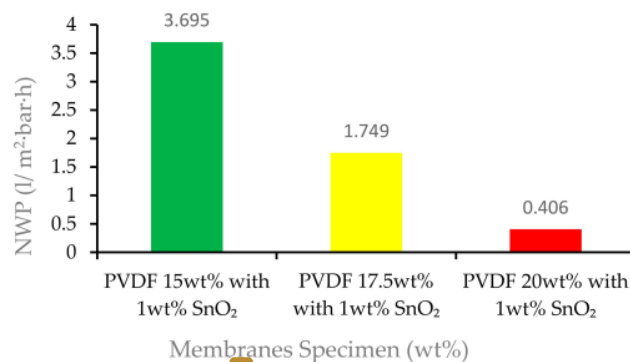
Figure 10. Average NWP of 15 wt%, 17.5 wt%, and 20 wt% PVDF with 1% tin dioxide membranes.
