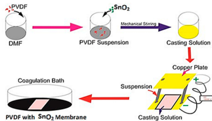
Figure 2. PVDF and tin dioxide membrane manufacturing process.
