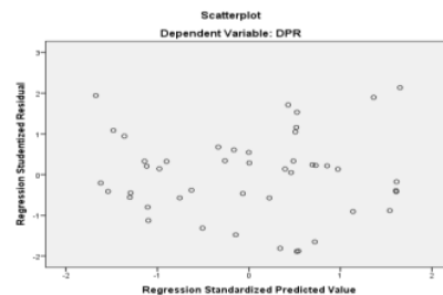
Heteroscedasticity Test Results
