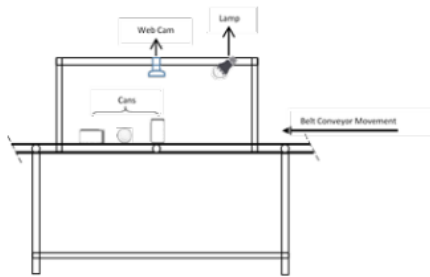
Figure 1. The cans image capturing system
