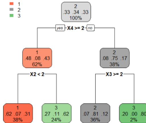
Fig. 2. Tree structure using discretization into two categories
