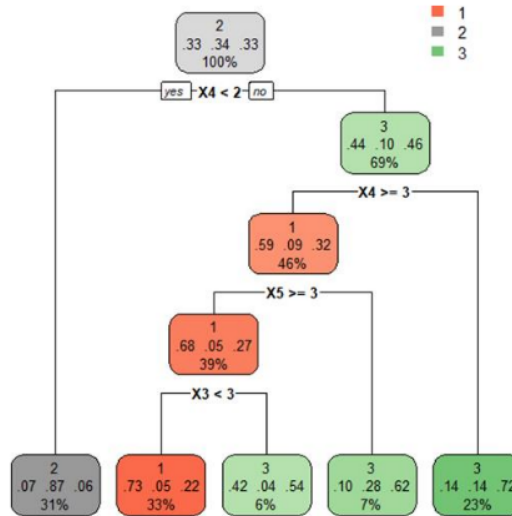
Fig. 3. Tree structure using discretization into three categories
