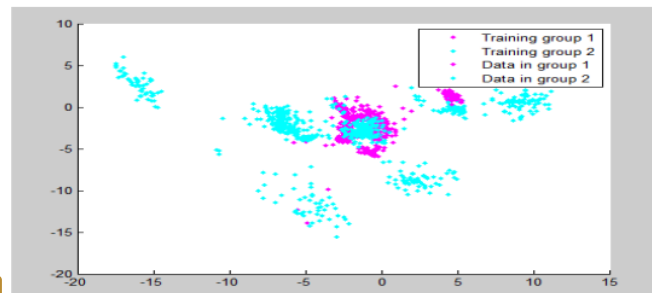
6 FIGURE 3. Scatter diagram show classification for dimensionality 50 and k=3
