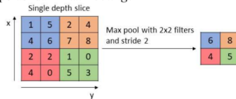
Gambar 3. Contoh Operasi Max Pooling
