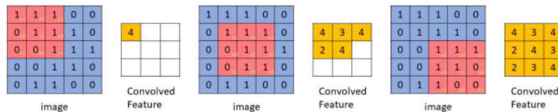
Gambar 2. Proses Convolution Layer
