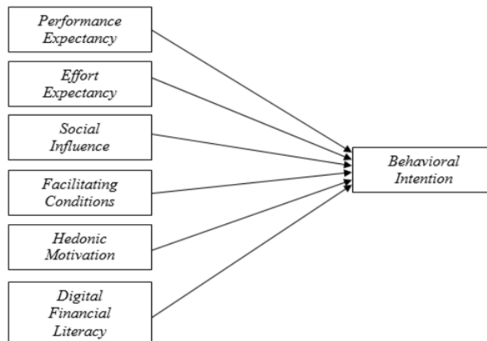
Figure 1. Framework
