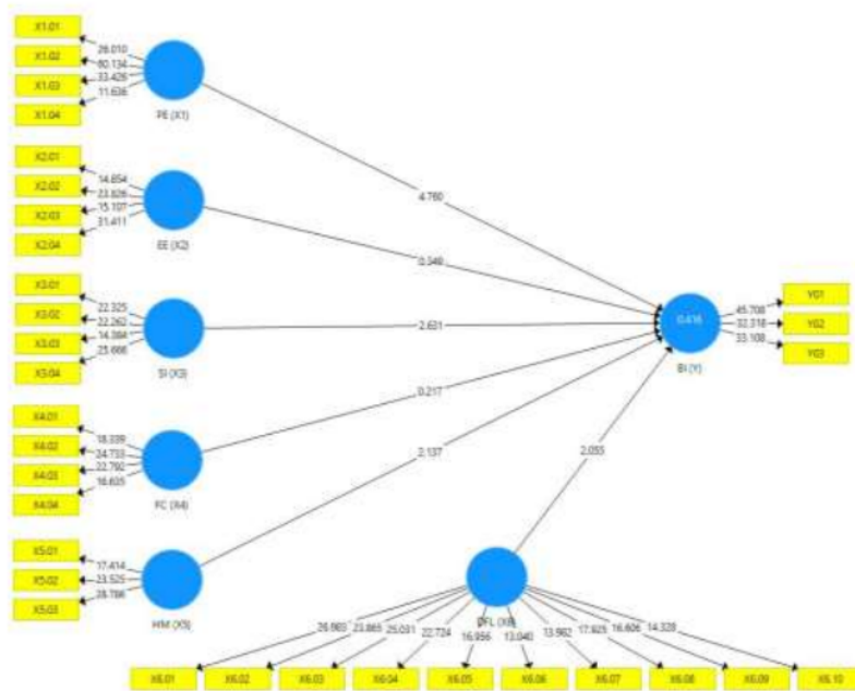
Figure 2. T-Statistic
