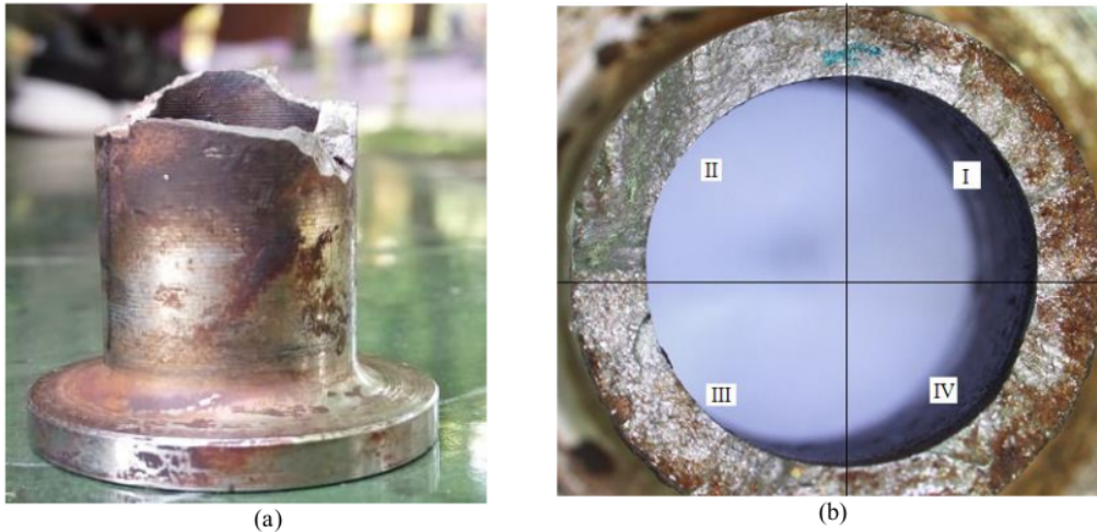
Figure 1. Fracture Morphology
