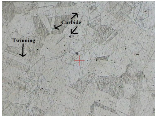
Figure 4. Microstructure observation
