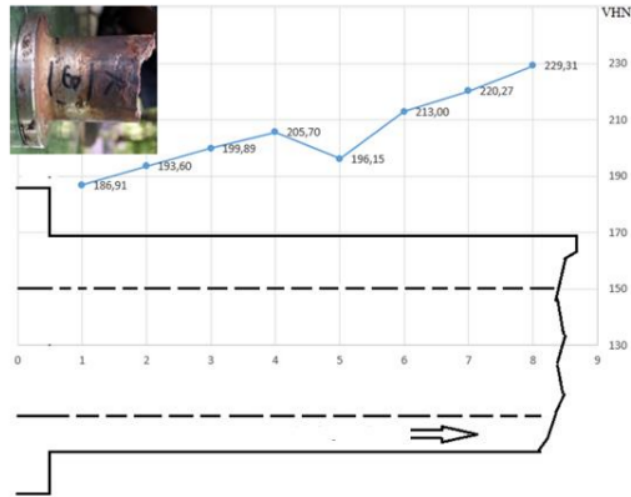
Figure 2. Vickers hardness test result
