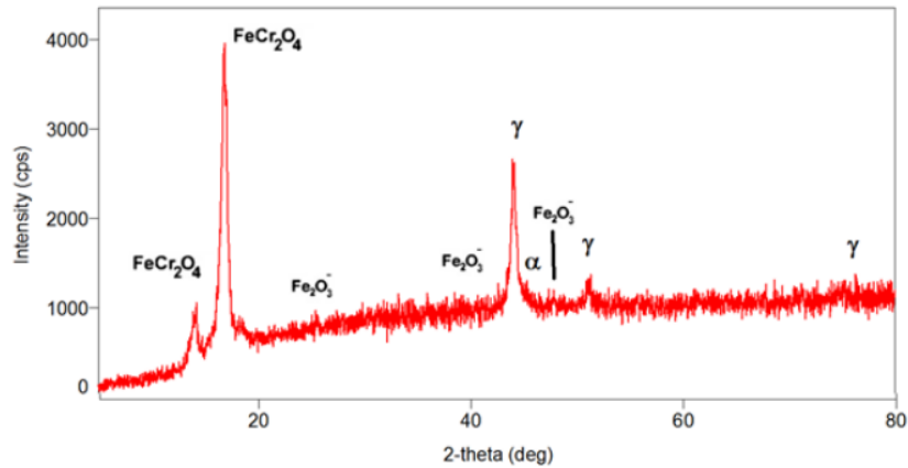
Figure 3. XRD test result
