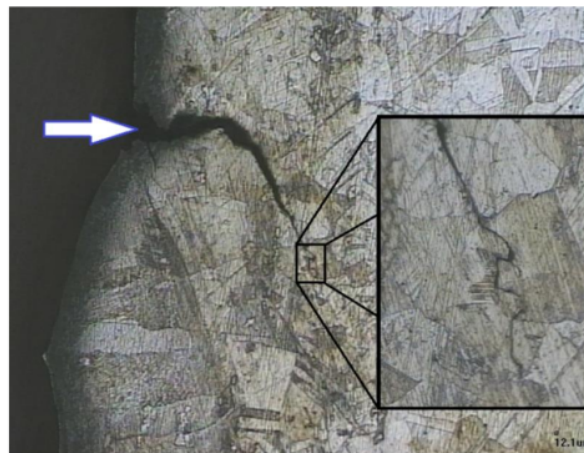
Figure 6. The propagation of inter-granular corrosion
