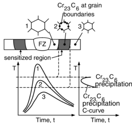
Figure 5. SS 304 sensitization zone
