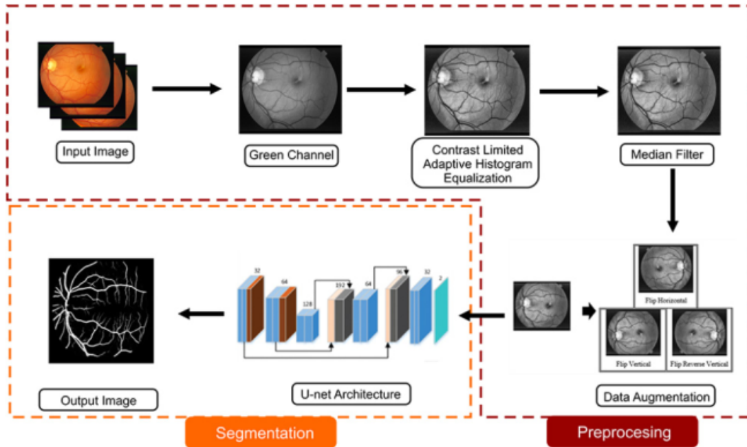
1 Fig. 1. Flowchart of the proposed method for data augmentation on vascular retinal image segmentation.
