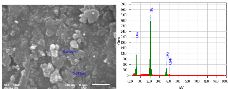
Figure 3. SEM micrograph and EDS spectra of nano-hydroxyapatite
