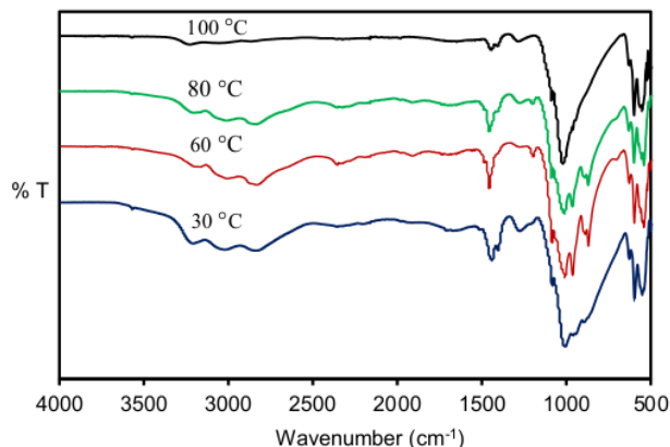
Figure 2. FTIR spectra of nano-hydroxyapatite
