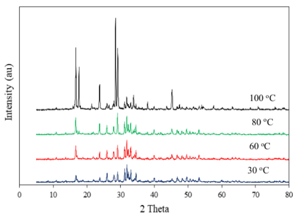
Figure 1. XRD spectra of nano-hydroxyapatite
