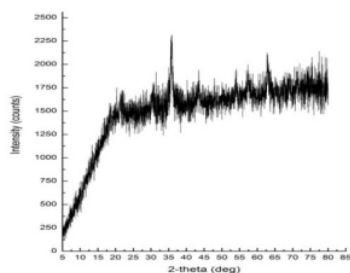
Figure 3. XRD pattern of Magnetite Nanoparticles
