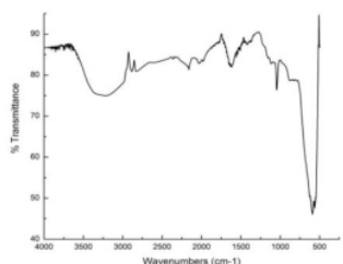
Figure 5. FT-IR analysis of \text{SnO}_2\text{-Fe}_3\text{O}_4
