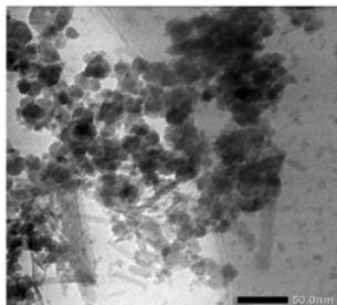
Figure 6. TEM images of \text{SnO}_2\text{-Fe}_3\text{O}_4
