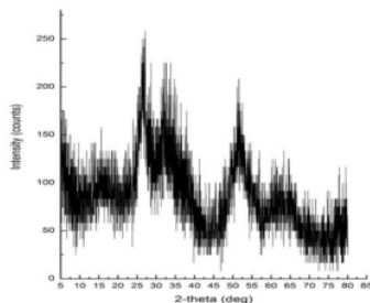
Figure 1. Diffractogram of \text{SnO}_2
