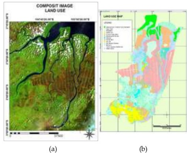
Fig. 3. (a) composite TM8 Image 5-4-2 band and (b) Classification of land use map
