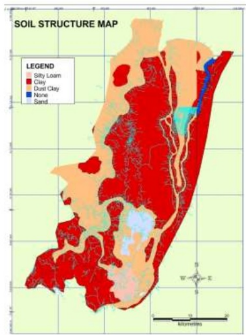
Fig. 4. Extract composite TM 8 Image with NDSI Method for Classification of Soil structure
