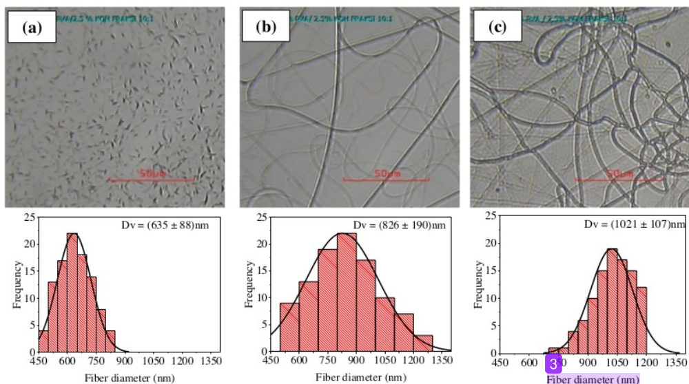
Figure 4. Morphology and diameter distribution of nanofiber (a) PK 1, (b) PK 2, and (c) PK 3.
