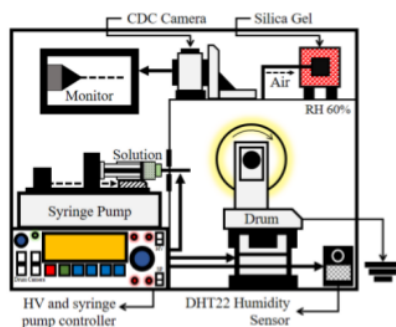
Figure 1. Schematic illustration of electrospinning apparatus.
