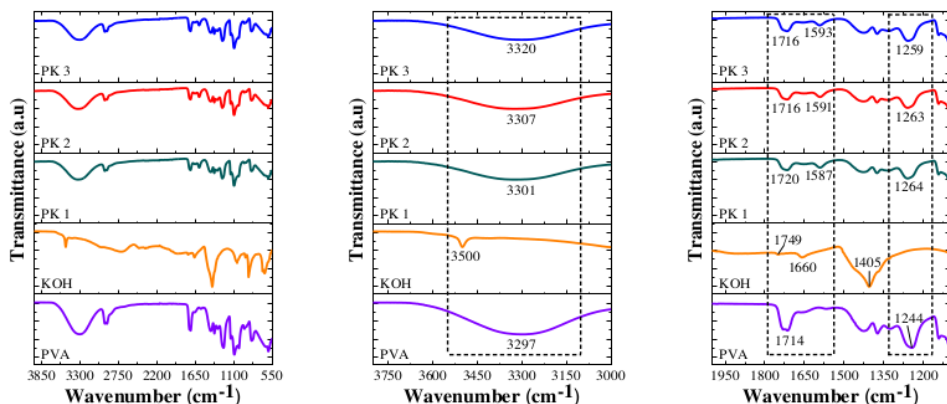
Figure 7. FTIR spectra of PVA/KOH PK 1, PK 2 and PK 3 nanofiber.
