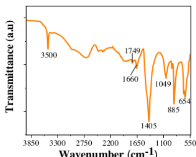
Figure 6. FTIR spectrum of Potassium hydroxide (KOH).
