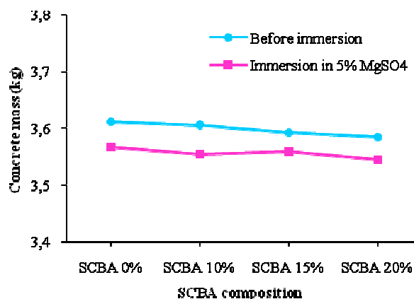
Fig. 7 The effect of SCBA content on concrete mass with w/c = 0.325 ( MgSO_4 = 5\% )
