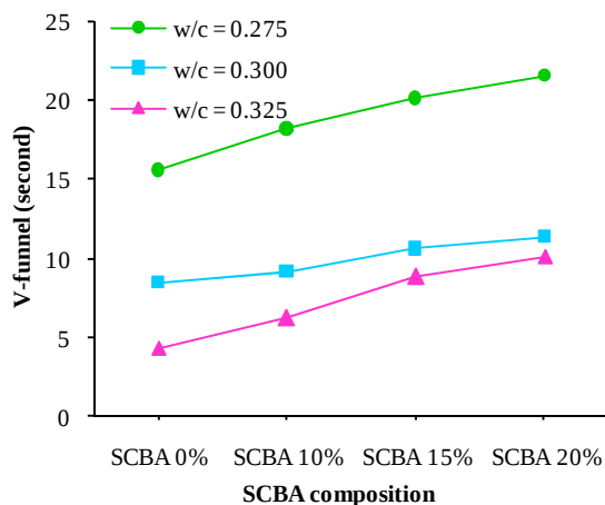
Fig. 3 The effect of SCBA on V-funnel
